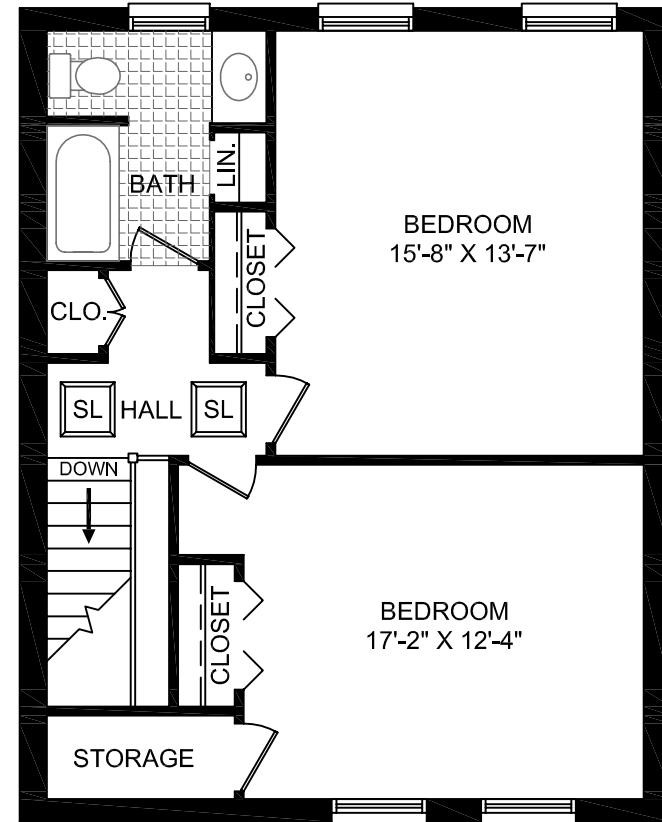
SECOND FLOOR
